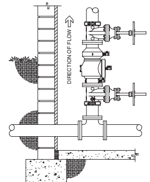
VERTICAL INSTALLATION (3500SYG)
