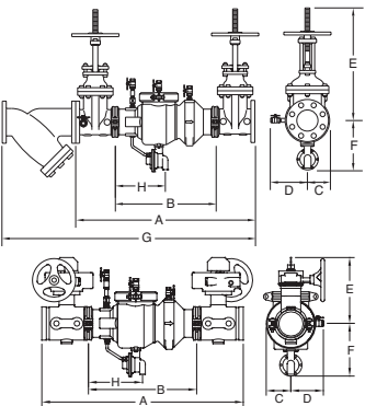
MODEL 375A with BG option
